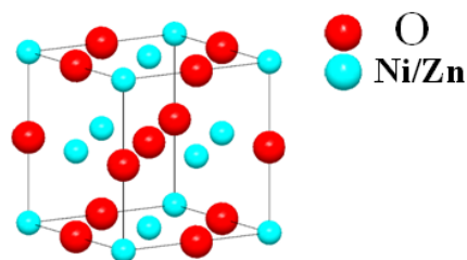
Figure 1: Cubic unit cell for Zn_xNi_{1-x}O
